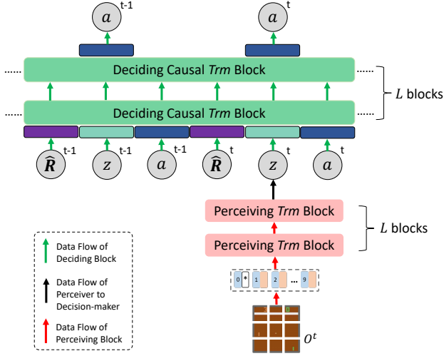
Figure 3: The architecture of the proposed Vanilla-PDiT.
